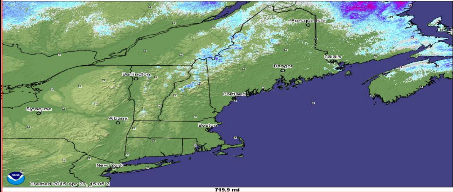
Modeled Snow water Equivalent forecasted for 2015 April 28, 12:00 UTC
