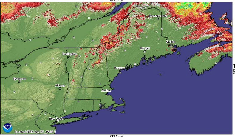
Modeled Snow Water Equivalent forecasted for 2015 April 28, 12:00 UTC
