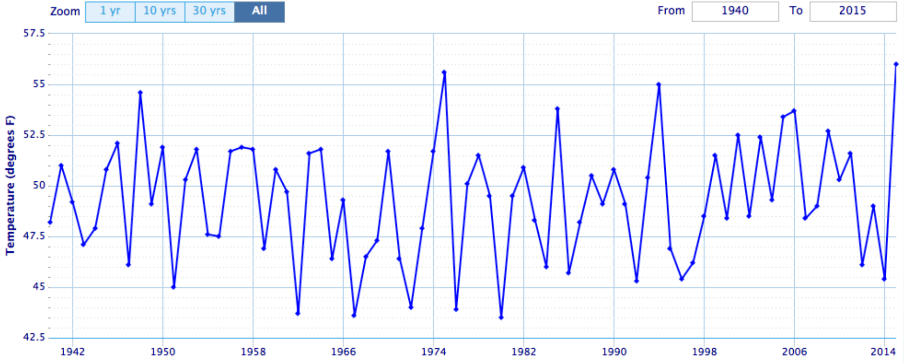
Mean Avg Temperature Nov 1 to Nov 22 – NEW YORK LAGUARDIA AP, NY
