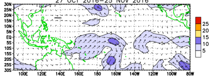
CDAS 200-hPa Wind Anoms 27 OCT 2016-25 NOV 2016
