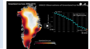
Video: Greenland ice loss 2002-2016
