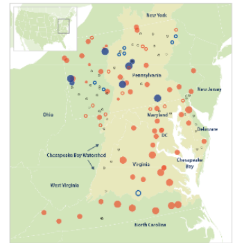
Changes in Stream Water Temperatures in the Chesapeake Bay Region, 1960-2014
